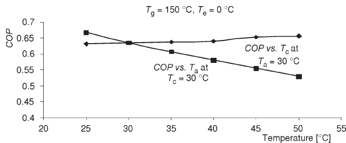
Figure 7. Effect of condenser and absorber Temperature on COP at T_g = 150\text{ }^\circ\text{C}
