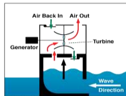
Fig. 6 Oscillating Water Column (OWC) Type Wave Energy Converter
