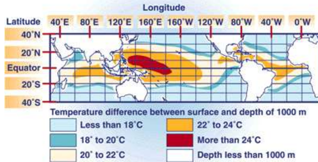
Fig. 3 Temperature difference of seawater between surface and depth of 1000 m
