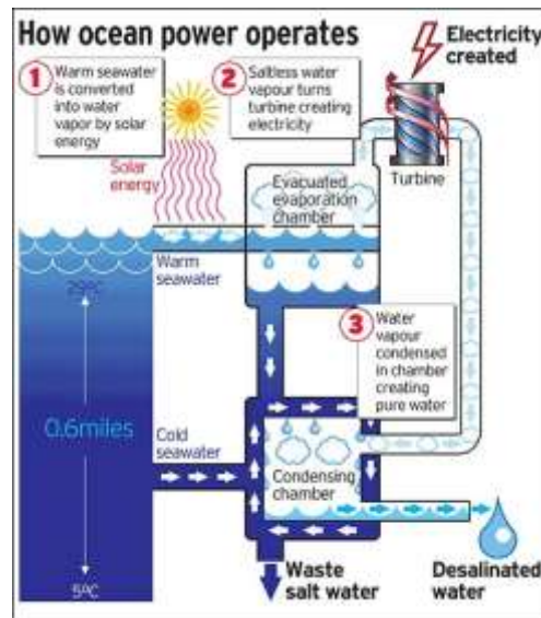
Fig. 4 Open cycle OTEC system
