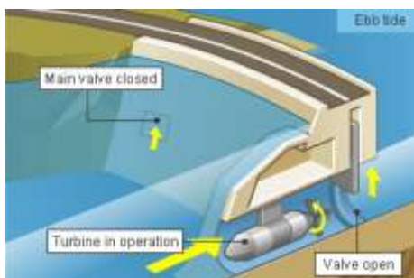
Fig.9 Power generation during ebb tide
