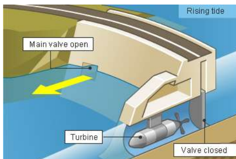
Fig.8 Water entering into the reservoir during rising tide
