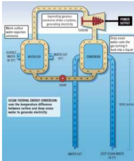
Fig. 5 Closed cycle OTEC system
