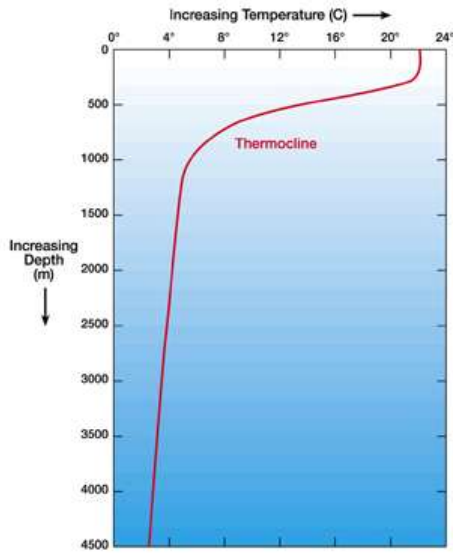
Fig.2 Thermocline in the ocean
