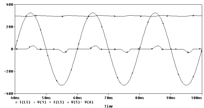
Fig. 1b. Source current and capacitor voltage wave forms.
