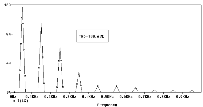
Fig. 1c. Harmonic spectrum of the source current waveform.
