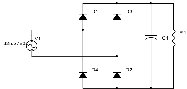
Fig. 1a. Circuit diagram of single - phase diode bridge rectifier.
