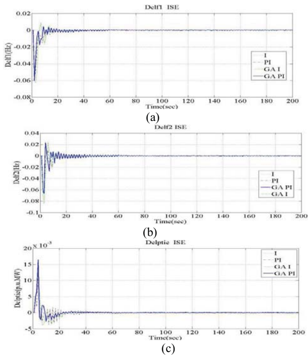
Fig.3. Comparison of integral and PI controller responses with 1% step load perturbation in hydrothermal area with ISE. (a) \Delta f_1=f(t) , (b) \Delta f_2=f(t) and (c) \Delta p_{tie}=f(t) .
