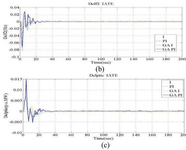
Fig.2. Comparison of integral and PI controller responses with 1% step load perturbation in hydrothermal area with IATE. (a) \Delta f_1=f(t) , (b) \Delta f_2=f(t) and (c) \Delta p_{tie}=f(t) .
