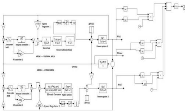
Fig.1. Transfer function model of an interconnected two area hydrothermal system with ISTE Optimum Technique
