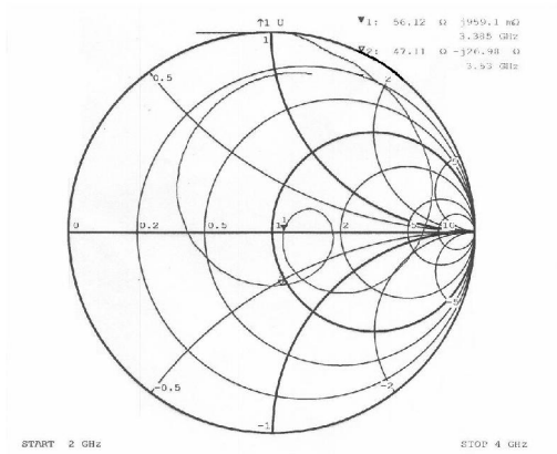
Figure 8. Measured input impedance of antenna
