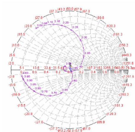
Figure 9. Simulated input impedance of antenna
