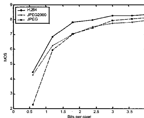
Fig. 2 Subjective Quality
